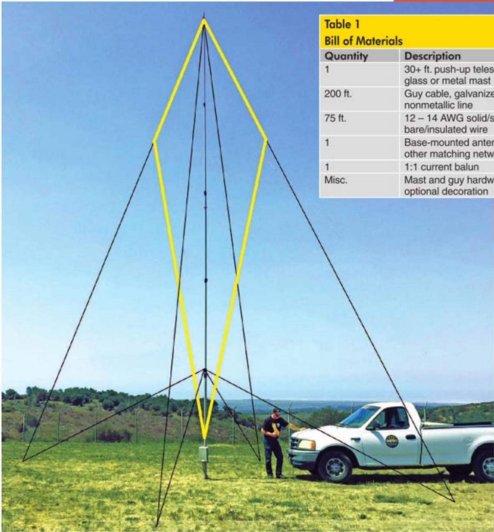
Figure 1 — The kite-shaped loop vertical installed at my radio club site. Loop wires are emphasized in yellow and the guy wires are shown in black.
